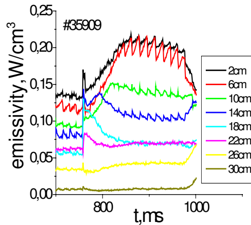
Fig.2 Temporal evolution of emissivity.
