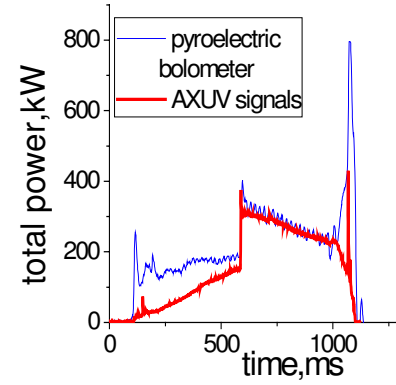
Fig.1. The total radiated power in the presence of iron traces.
