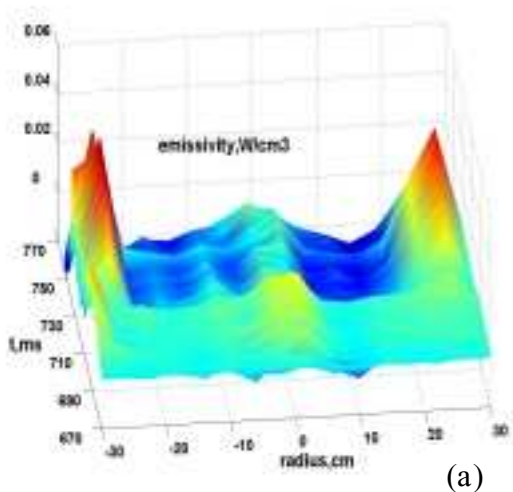
Fig.4. #35841 (H-like mode). (a)-temporal evolution of emissivity profiles; (b)-emissivity, electron temperature and density traces.
